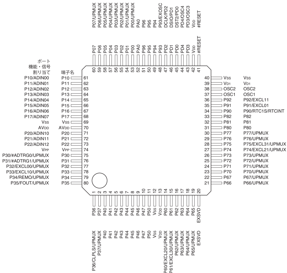
図1.3.1.2 S1C17589端子配置図 (QFP14-80PIN)
