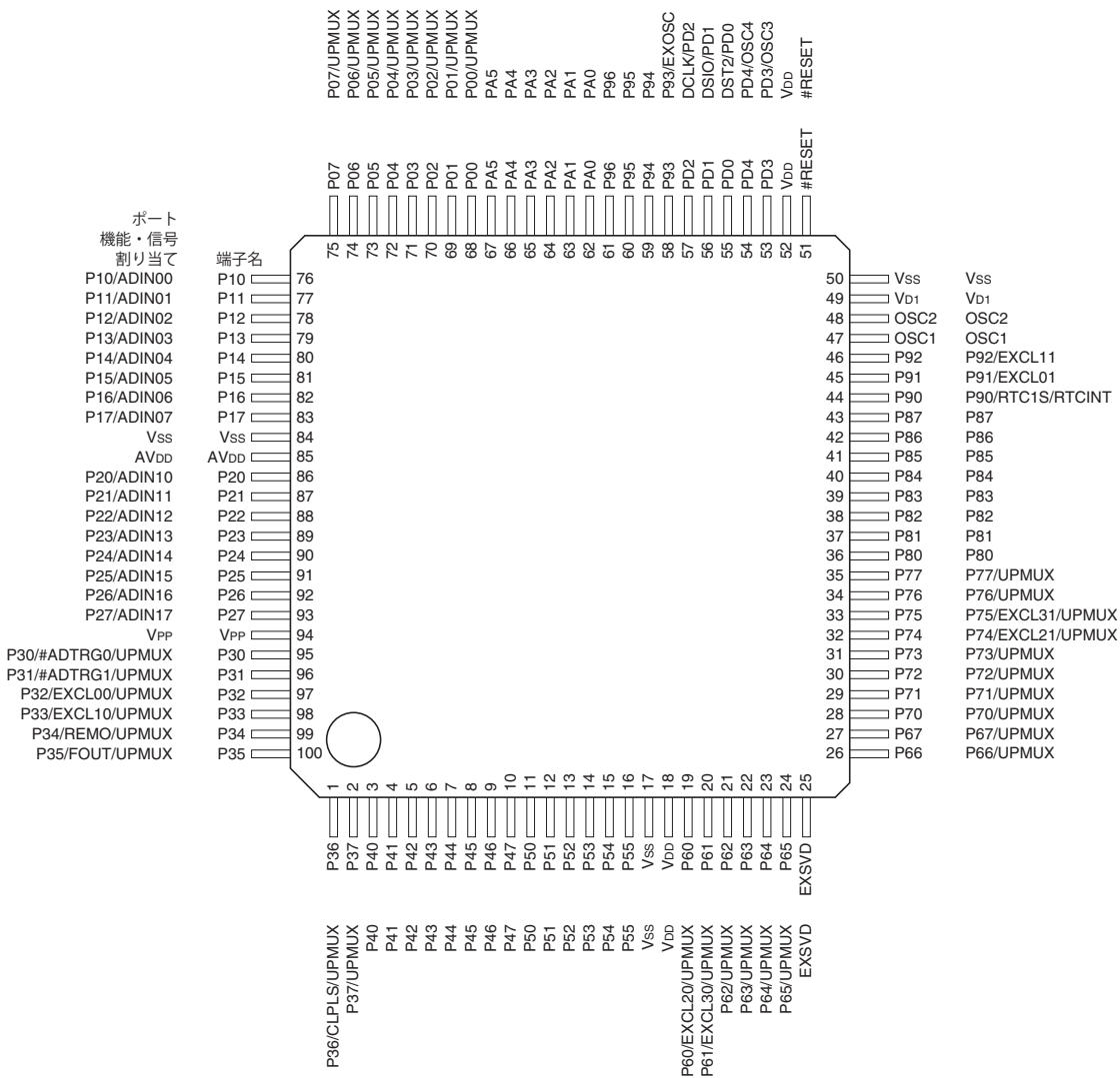
図1.3.1.1 S1C17589端子配置図 (QFP15-100PIN)
