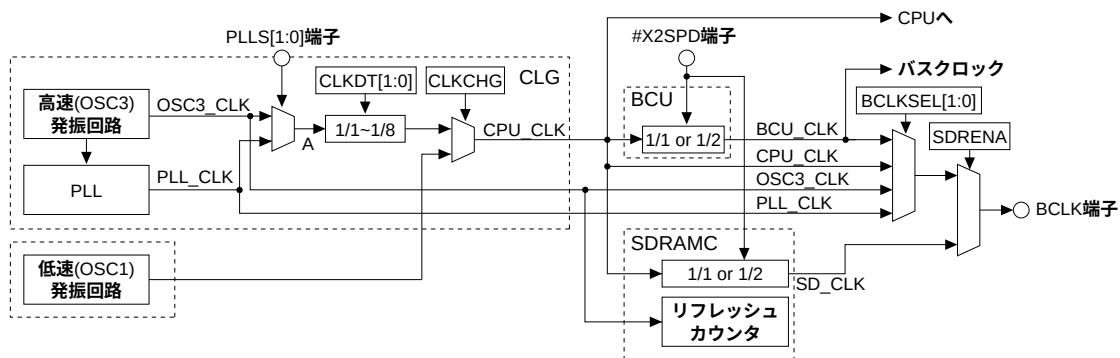
PLL_CLKとCPU_CLK
