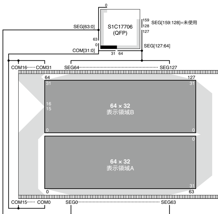
例2: COMPOS = 1, COMREV = 0, SEGREV = 1, LDUTY[2:0] = 0x4 (1/32デューティ, Type A)
