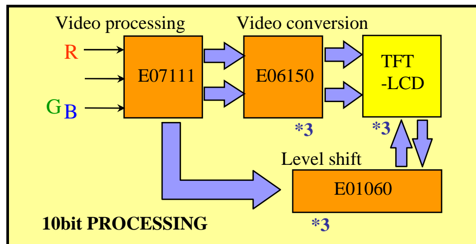
IC Block Diagram
