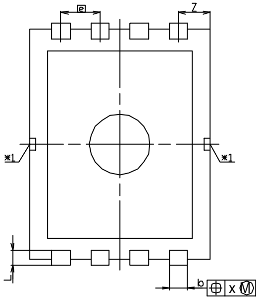
Bottom View
