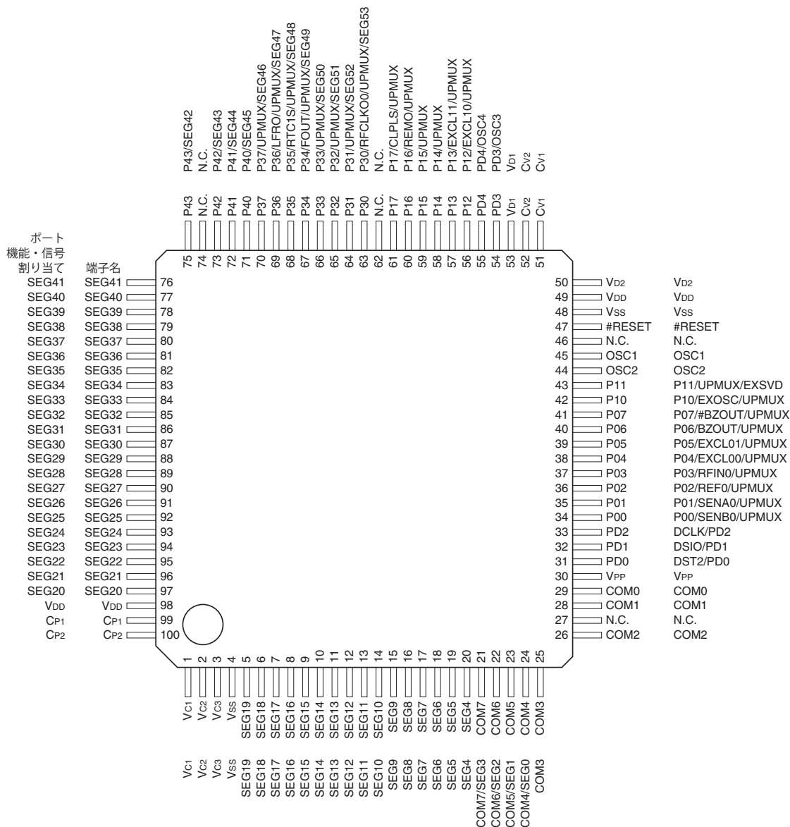
図1.3.1.1 S1C17W14端子配置図(QFP15-100PIN)
