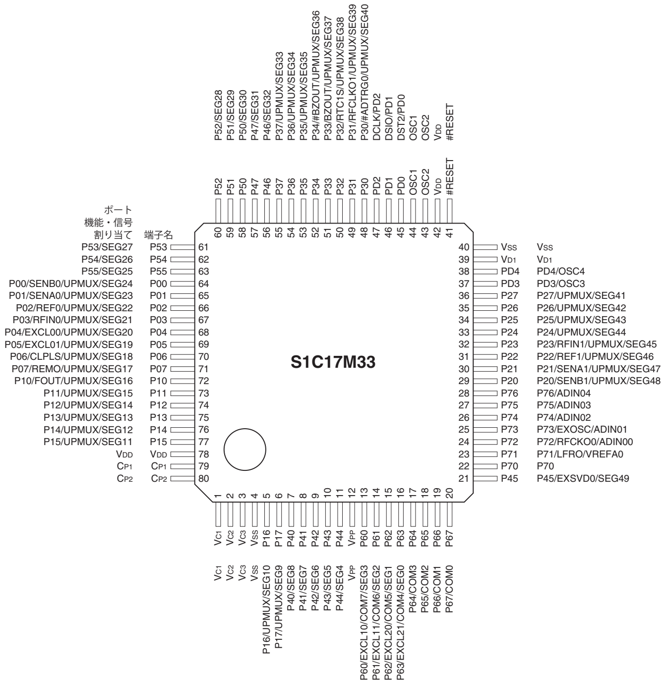
S1C17M33 端子配置図 (QFP14-80PIN)
