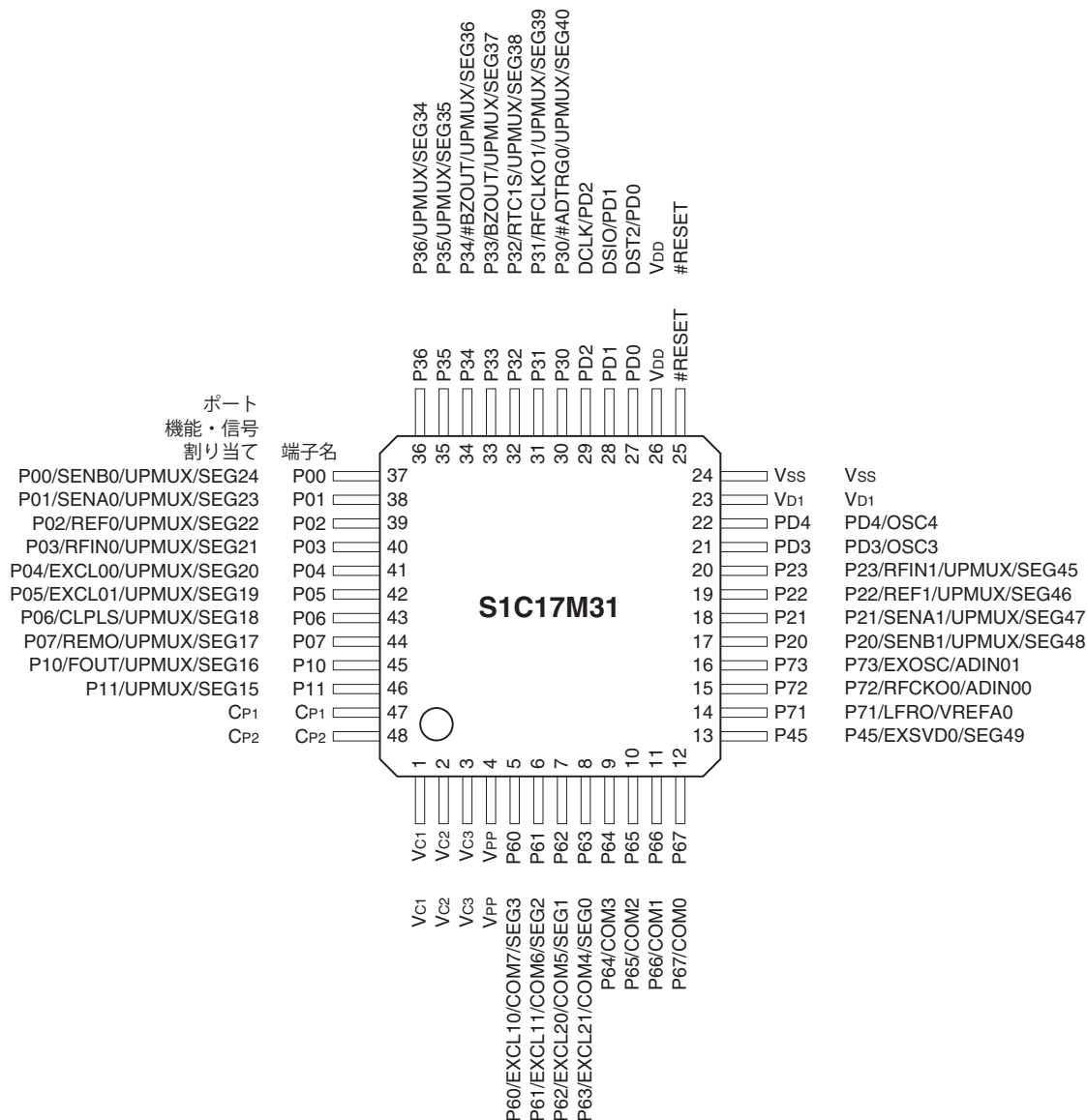
図1.3.2.1 S1C17M31端子配置図(TQFP12-48PIN)
