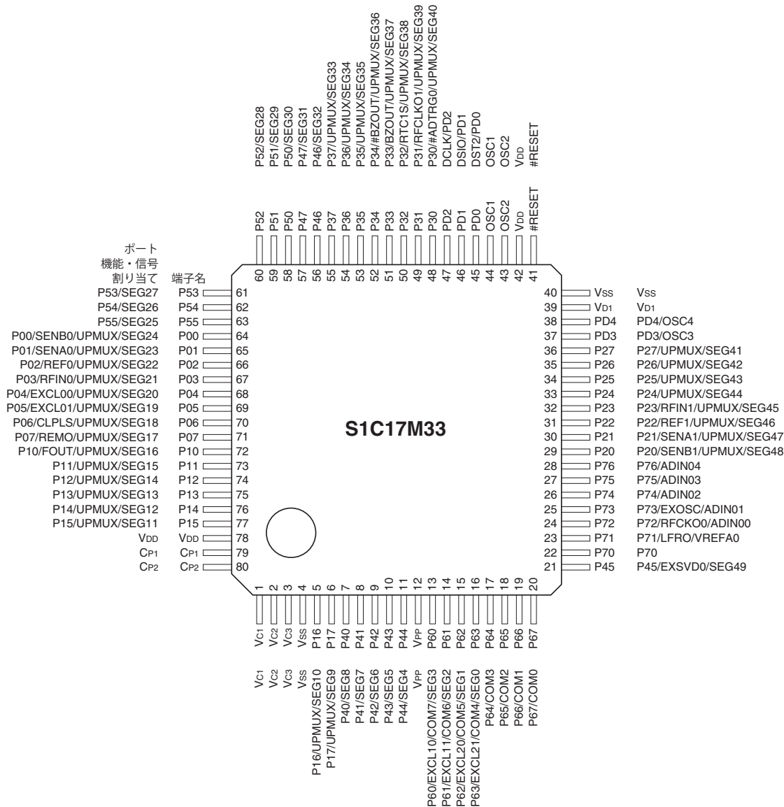
図1.3.4.1 S1C17M33端子配置図(QFP14-80PIN)
