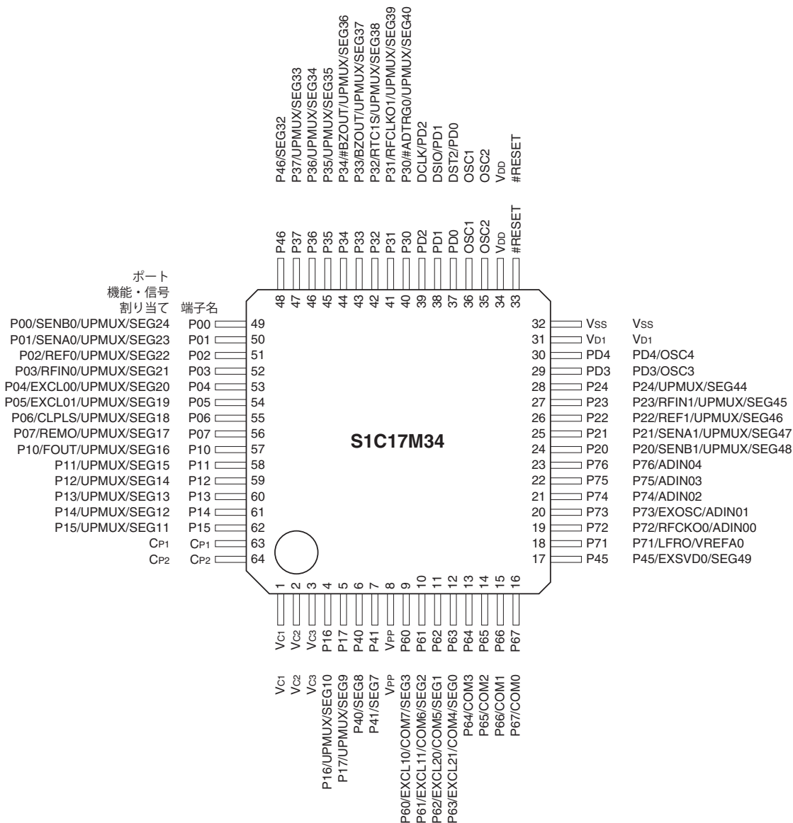
図1.3.6.1 S1C17M34端子配置図(TQFP13-64PIN)
