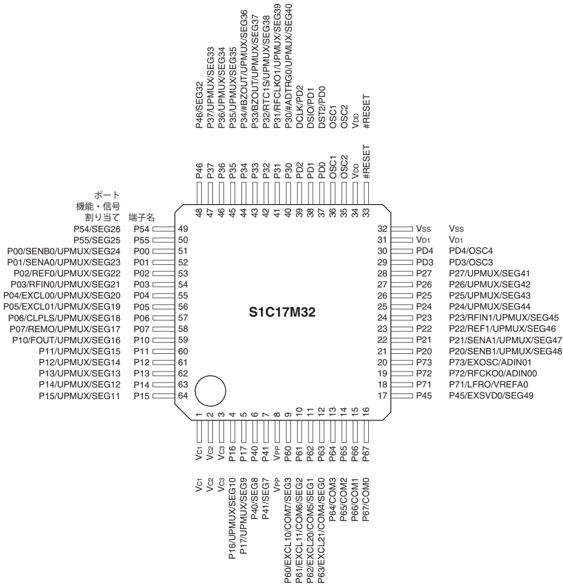
図1.3.3.1 S1C17M32端子配置図(TQFP13-64PIN)
