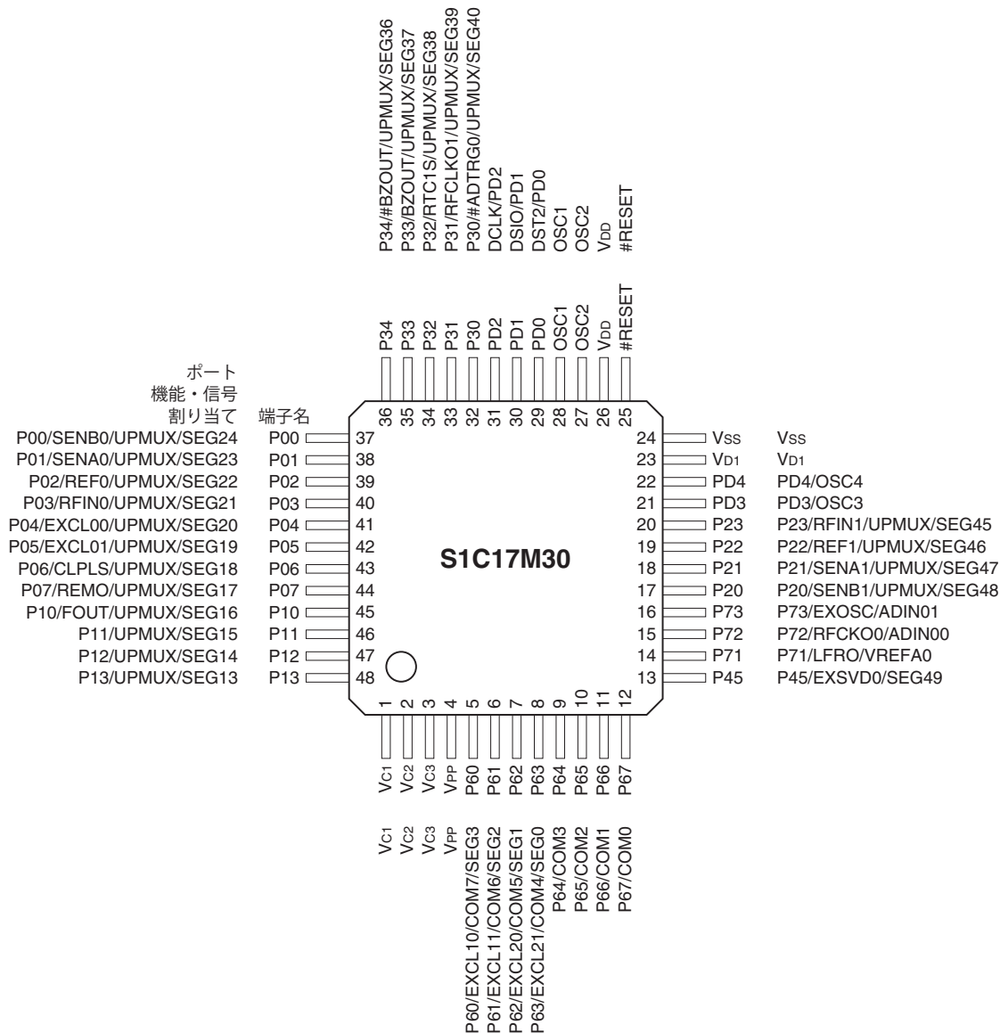
図1.3.1.1 S1C17M30端子配置図(TQFP12-48PIN)
